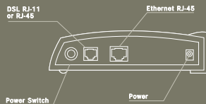
SpeedStream® 5251
